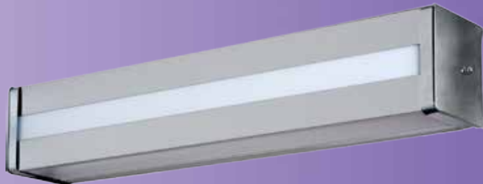
DEV Cutoff, Polished Aluminum Smooth White Acrylic Length: 24 1/4", 36 1/4", 48 1/4" Height: 4 1/2" Depth: 4 3/8"
